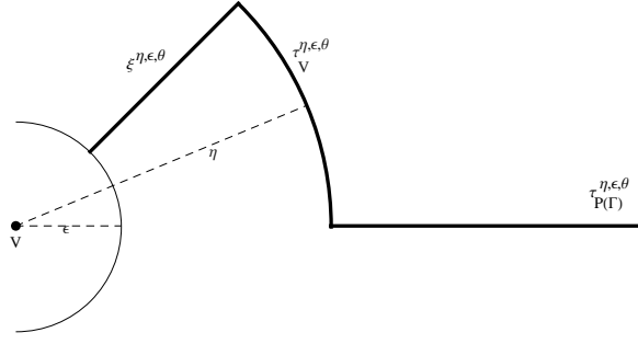
FIGURE 10. The monodromy chain, with angular variable \theta .
