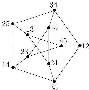
FIGURE 2. The Petersen graph \mathcal{G} . This is the graph with vertices corresponding to 2-element subsets of \{1, 2, 3, 4, 5\} , with two vertices \{i, j\} and \{k, \ell\} connected by an edge precisely when \{i, j\} \cap \{k, \ell\} = \emptyset . The graph \mathcal{G} is the intersection graph of the 10 lines on the quintic del Pezzo surface, with a vertex for each line and an edge connecting vertices corresponding to lines with nontrivial intersection.
