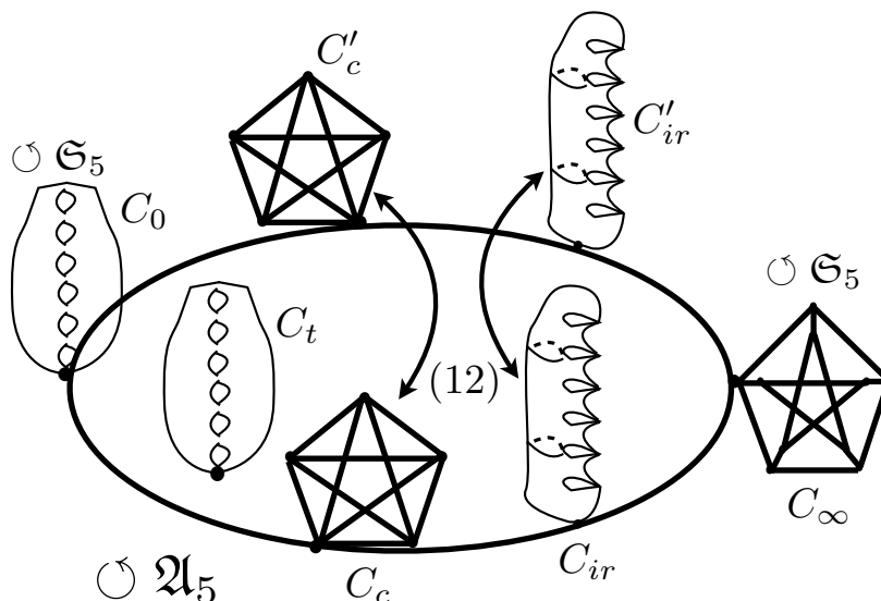
FIGURE 1. A schematic of the Wiman-Edge pencil \mathcal{C} , consisting of genus 6 projective curves containing the alternating group \mathfrak{A}_5 in their automorphism group. The generic curve C_t \in \mathcal{C} has \text{Aut}(C_t) \cong \mathfrak{A}_5 , while there is a unique smooth member C_0 \in \mathcal{C} , the Wiman sextic , with more symmetry: \text{Aut}(C_0) \cong \mathfrak{S}_5 . There are 5 singular members of \mathcal{C} : two irreducible curves, 6-noded rational curves C_{ir} and C'_{ir} ; two curves C_c and C'_c , each consisting of 5 conics whose intersection graph is the complete graph on 5 vertices; and a union C_\infty of 10 lines whose intersection graph is the Petersen graph. The group \mathfrak{S}_5 acts on \mathcal{C} with \mathfrak{A}_5 leaving each member of \mathcal{C} invariant. This action has two \mathfrak{S}_5 -invariant members, C_0 and C_\infty , while any odd permutation switches C_{ir} with C'_{ir} and C_c with C'_c .
