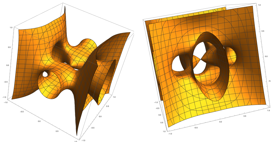
FIGURE 3. Two views of a piece of the Wiman sextic (the image of the Wiman curve in \mathbb{P}^2 ).
