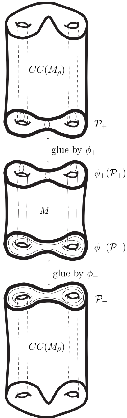
FIGURE 1. Constructing the manifold N
