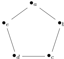
Figure 6: r = 1, n = 2
