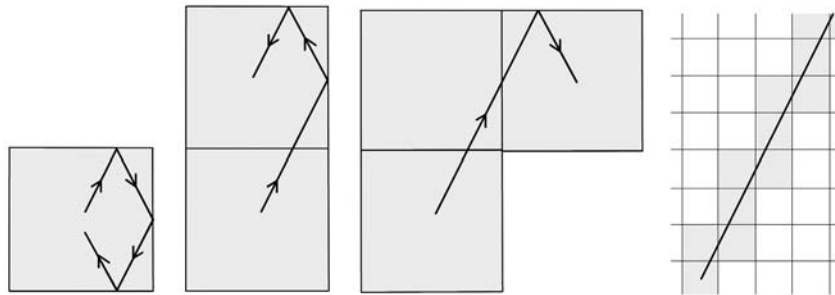
FIGURE 14. Unfolding billiards in a square to get lines in a torus (courtesy of Diana Davis, used with permission).
