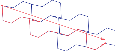
FIGURE 10. Closing up a ray that comes back close to itself (courtesy of Marcelo Viana, used with permission).
