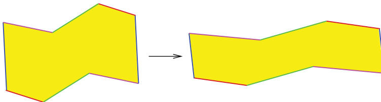
FIGURE 11. A local picture of the Teichmüller flow (courtesy of Marcelo Viana, used with permission).
