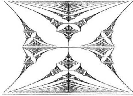
FIGURE 13. Hofstadter's butterfly. Reprinted figure with permission as follows: Douglas R. Hofstadter, Energy levels and wave functions of Bloch electrons in rational and irrational magnetic fields , Physical Review B 14 (1976), 2239–2249. Copyright 1976, American Physical Society.
