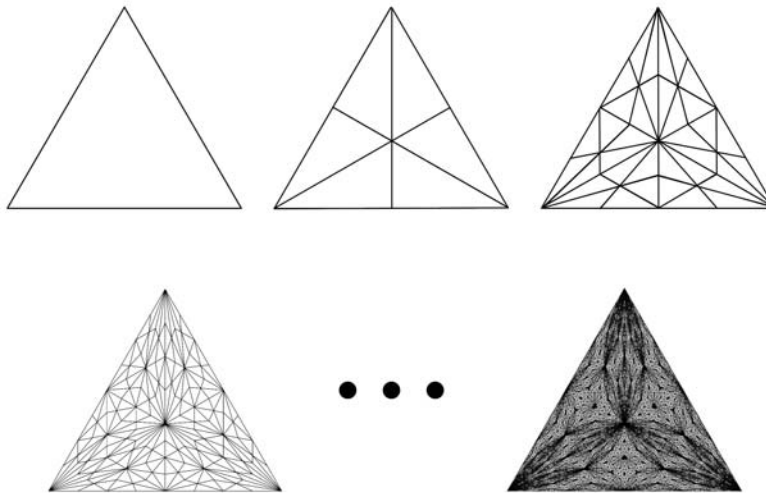
FIGURE 2. Iterating barycentric subdivision (courtesy of C. McMullen, [54], used with permission).
