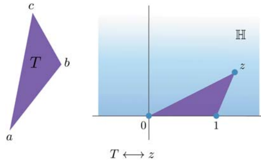
FIGURE 4. The upper half-plane \mathbb{H} is the space of marked triangles, up to Euclidean similarity. The triangle T on the left corresponds to the point z \in \mathbb{H} on the right.
