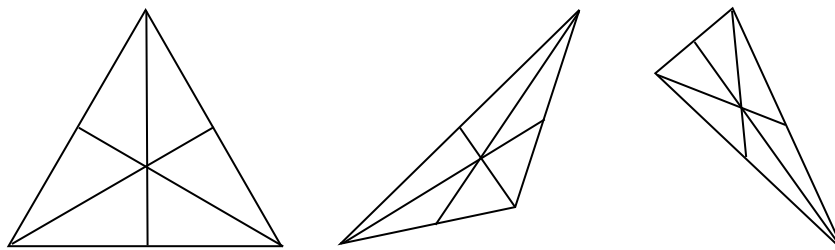
FIGURE 1. Barycentric subdivision.
