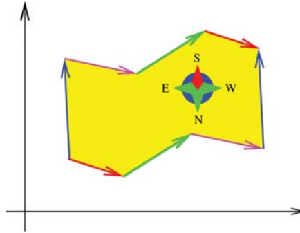
FIGURE 9. A flat surface (of genus 2) with a distinguished "South," also known as a translation surface. Parallel edges of the same color are identified (courtesy of Marcelo Viana, used with permission).
