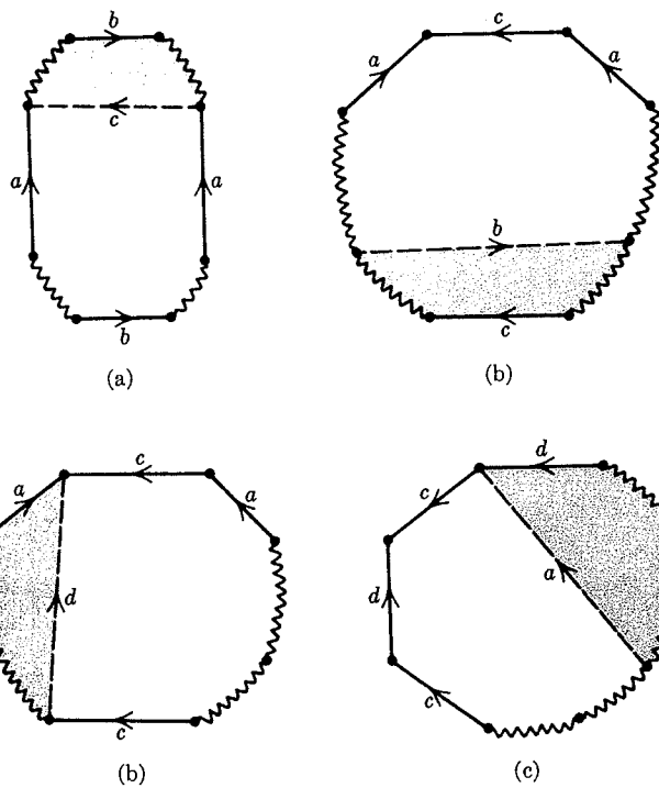
FIGURE 1.21. Fifth step in the proof of Theorem 5.1.
