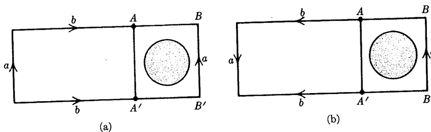
FIGURE 1.22. (a) Torus with hole. (b) Klein bottle with hole.
