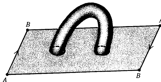
FIGURE 1.24. The result of cutting the spaces shown in Figure 1.23 along the line AB .
