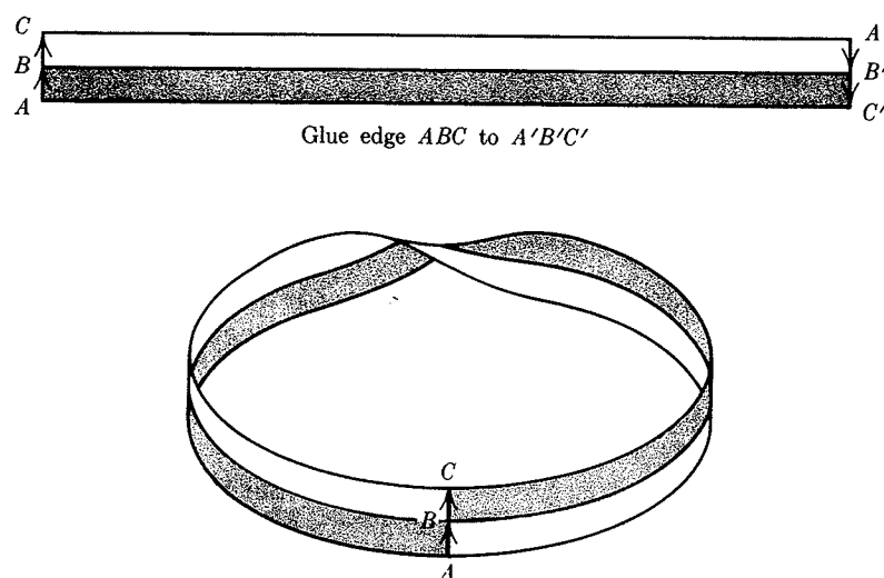
FIGURE 1.1. Constructing a Möbius strip.
