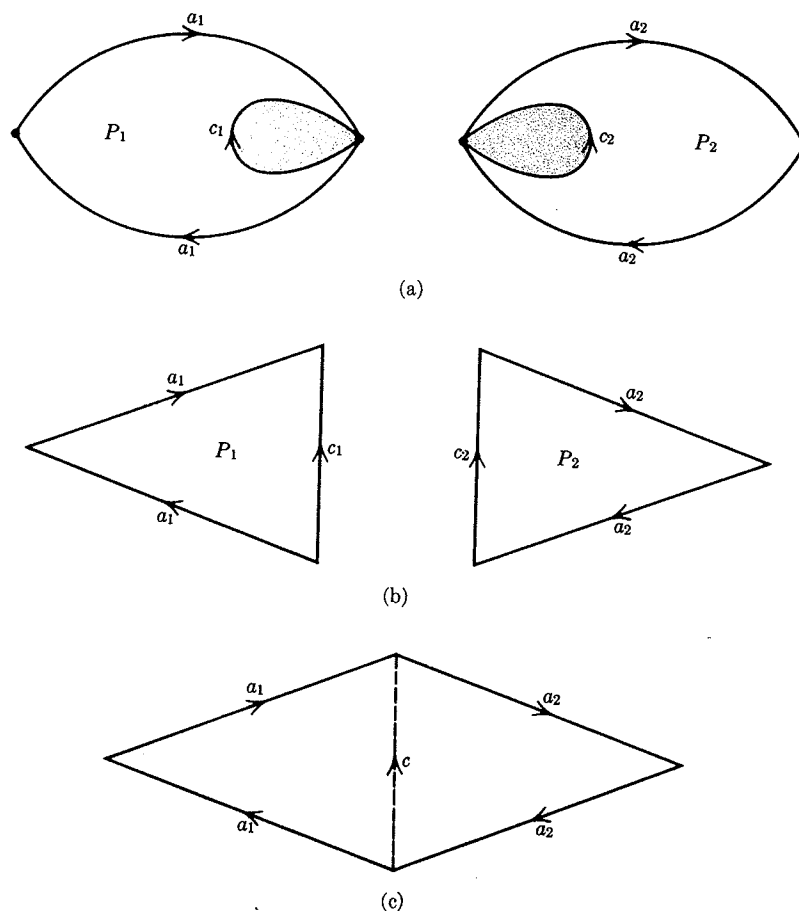
FIGURE 1.9. (a) Two disjoint projective planes, P_1 and P_2 . (b) Disjoint projective planes with holes cut out. (c) After gluing together.
