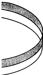
Möbius strip.
