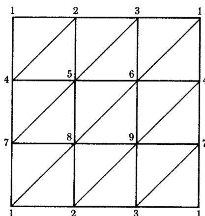
FIGURE 1.14. A triangulation of a torus.
