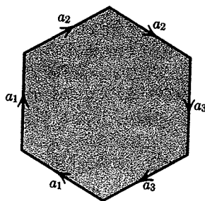
FIGURE 1.10. Construction of the connected sum of three projective planes by identifying the sides of a hexagon in pairs.
