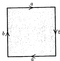
FIGURE 1.3. Construction of a projective plane from a square.
