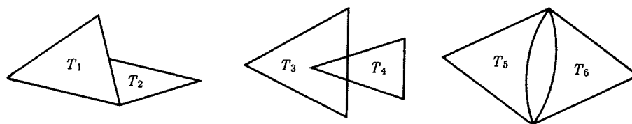
FIGURE 1.12. Some types of intersection forbidden in a triangulation.
